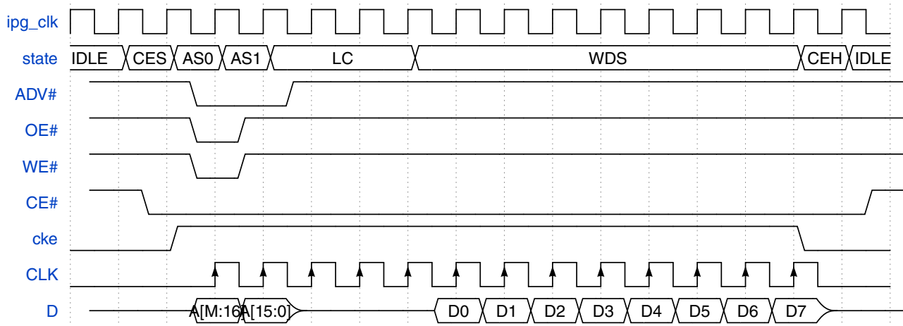
Figure 24-67. SRAM Write in SYNC mode (AADM)
