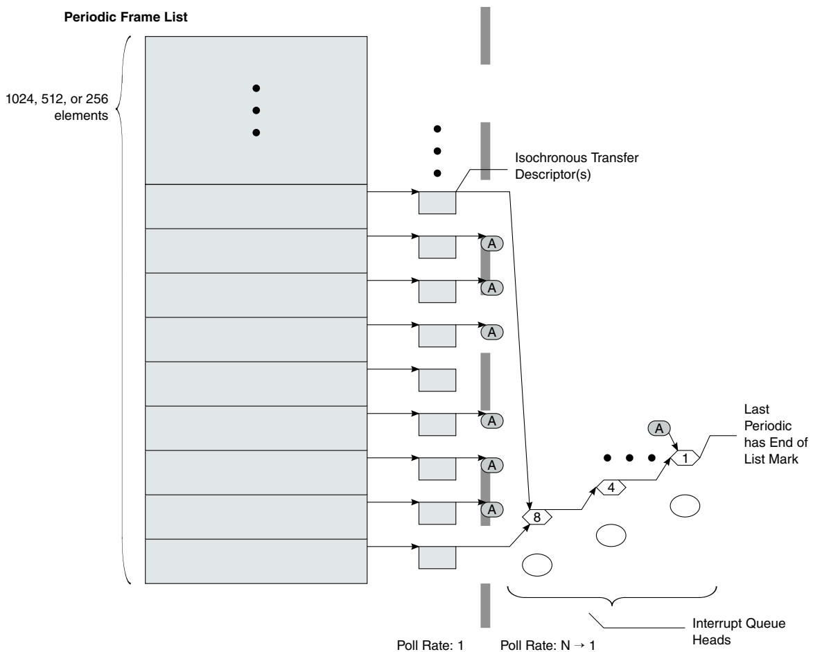
Figure 41-11. Example Periodic Schedule
