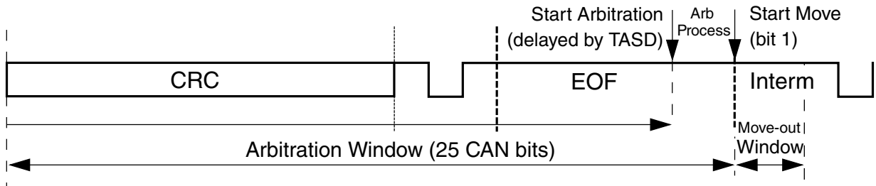
Figure 44-11. Arbitration and move-out time windows
