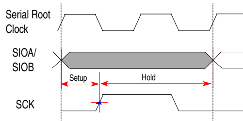
Figure 26-24. SDR instruction in DDR sequence
