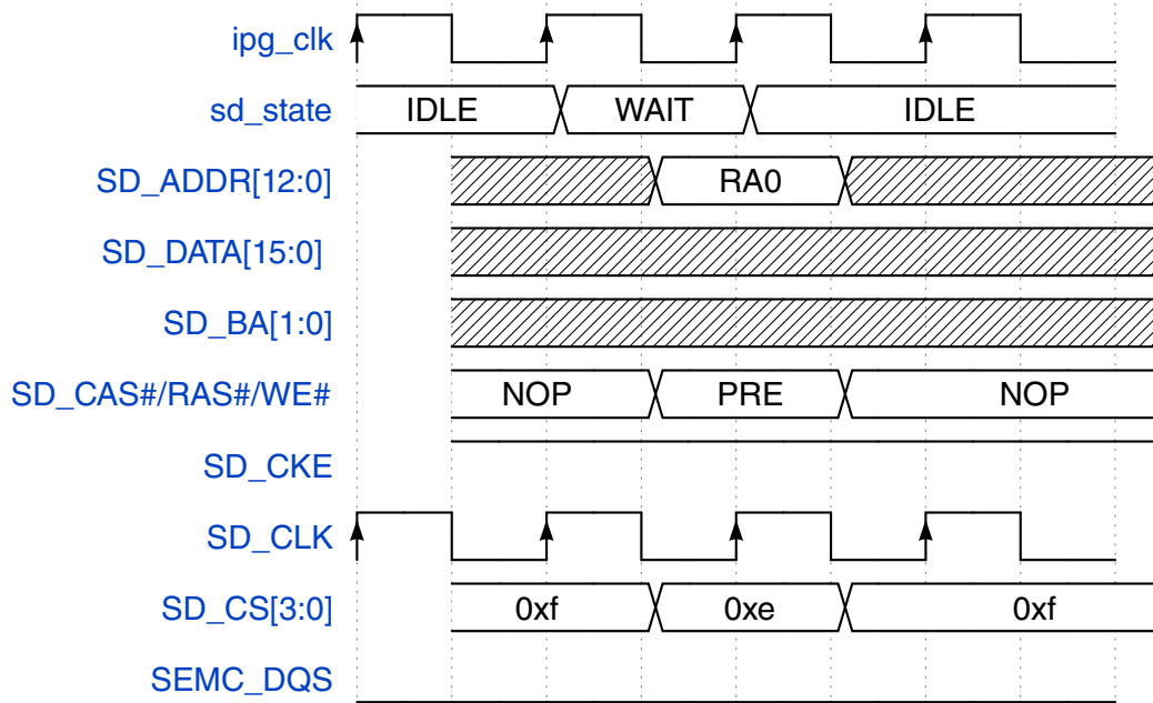
Figure 24-6. IP command - SDRAM PRECHARGE
