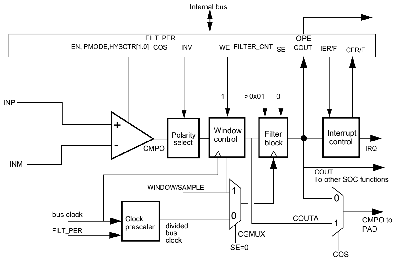
Figure 64-11. Windowed/Filtered mode
