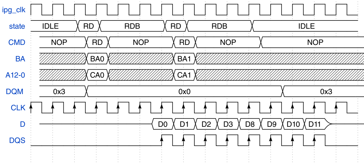
Figure 24-17. SDRAM Read-to-Read access (CL=3)
