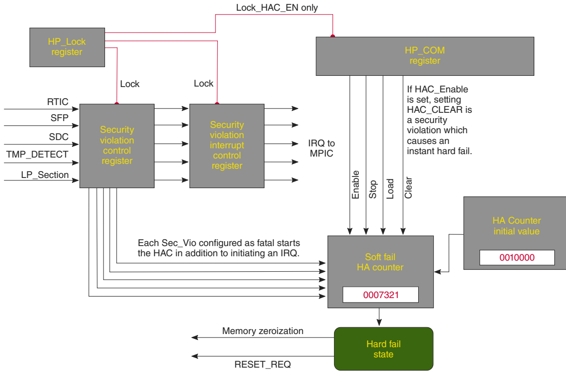
Figure 19-1. Relationship Between the Registers
