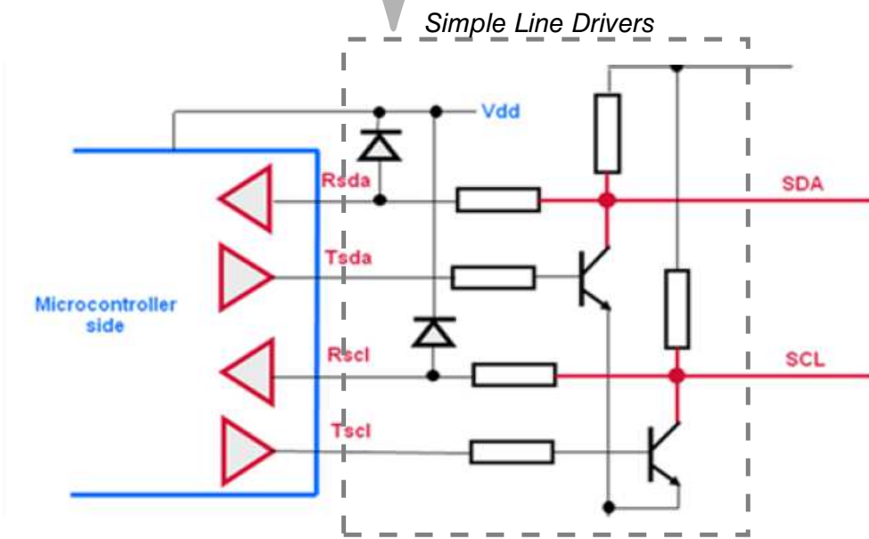
Figure 46-6. 4-Wire scheme
