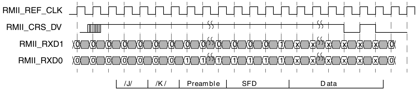
Figure 40-19. RMII receive operation
