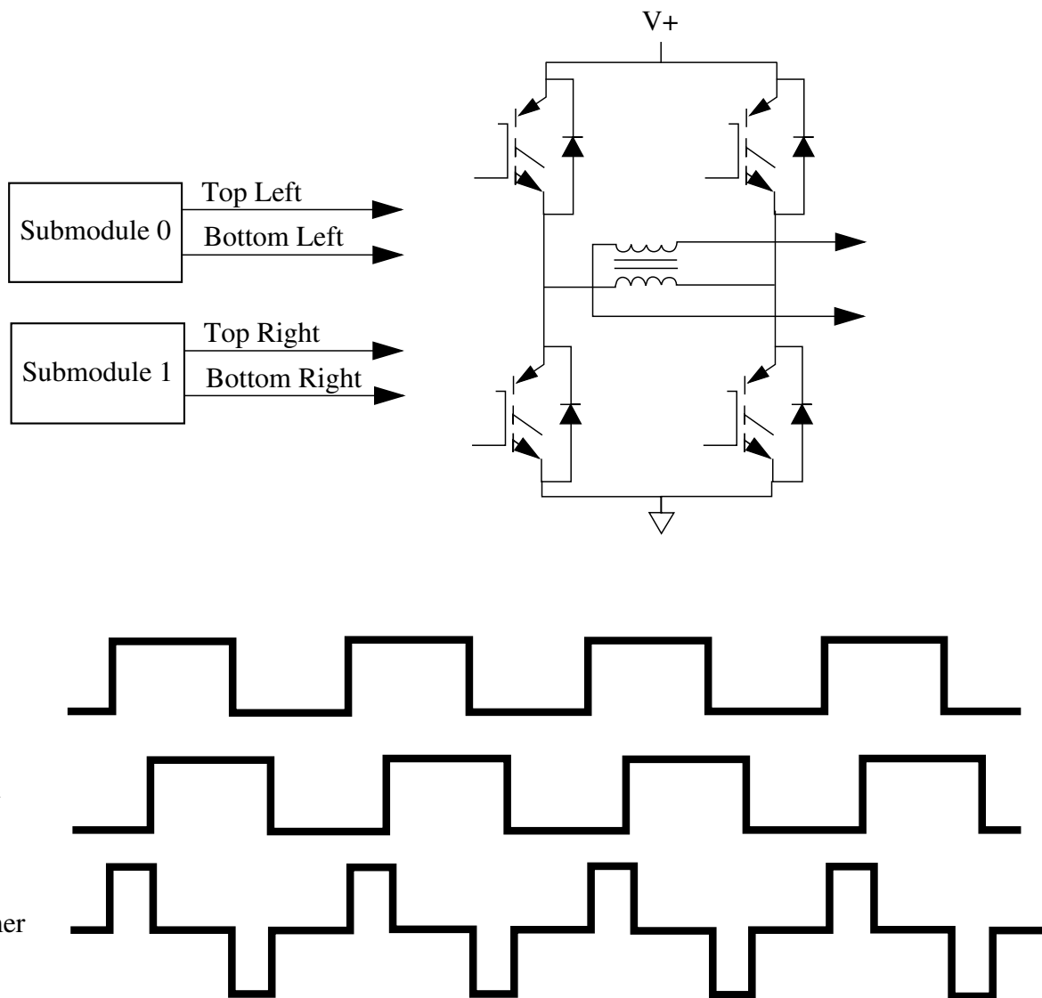
Figure 54-5. Phase Shifted PWMs Applied to a Transformer Primary
