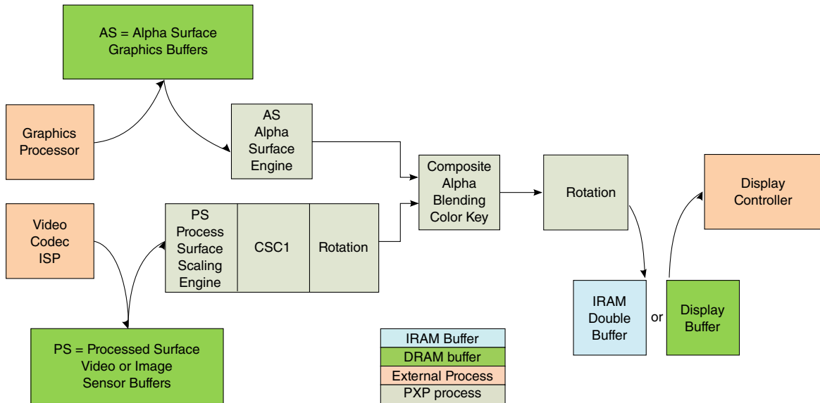
Figure 35-1. PXP Architecture
