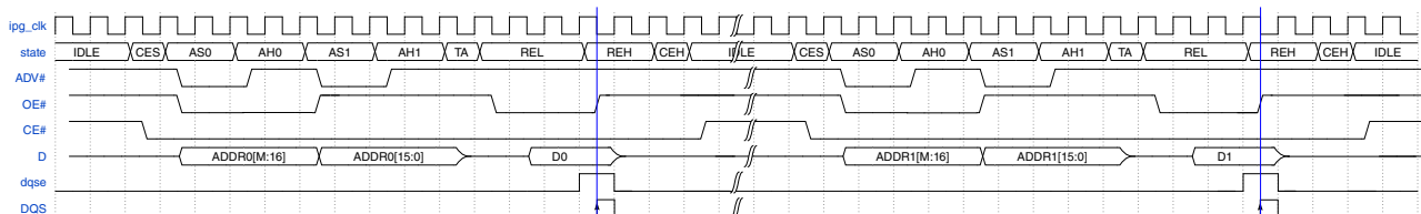
Figure 24-58. SRAM Read in ASYNC mode (AADM)
