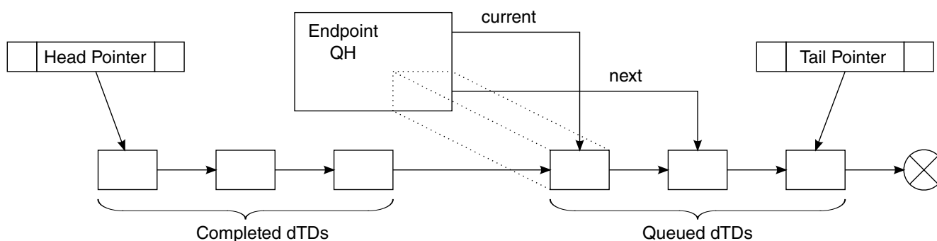
Figure 41-30. Software Link Pointers
