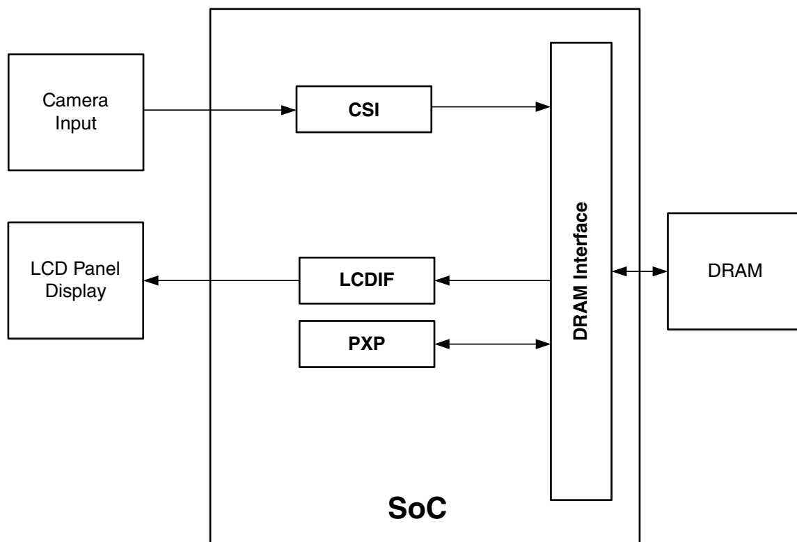
Figure 32-1. Block Diagram
