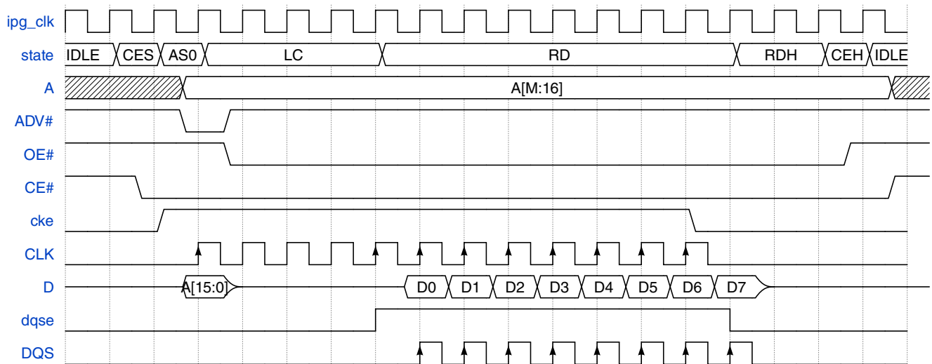
Figure 24-63. SRAM Read in SYNC mode (ADMUX)
