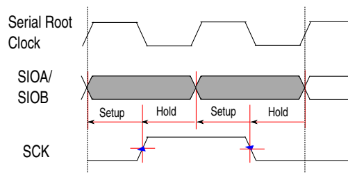
Figure 26-25. DDR instruction in DDR sequence
