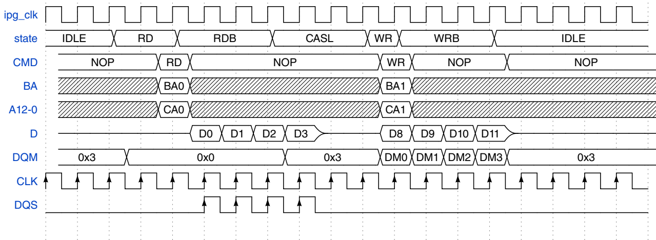
Figure 24-18. SDRAM Read-to-Write access (CL=1)
