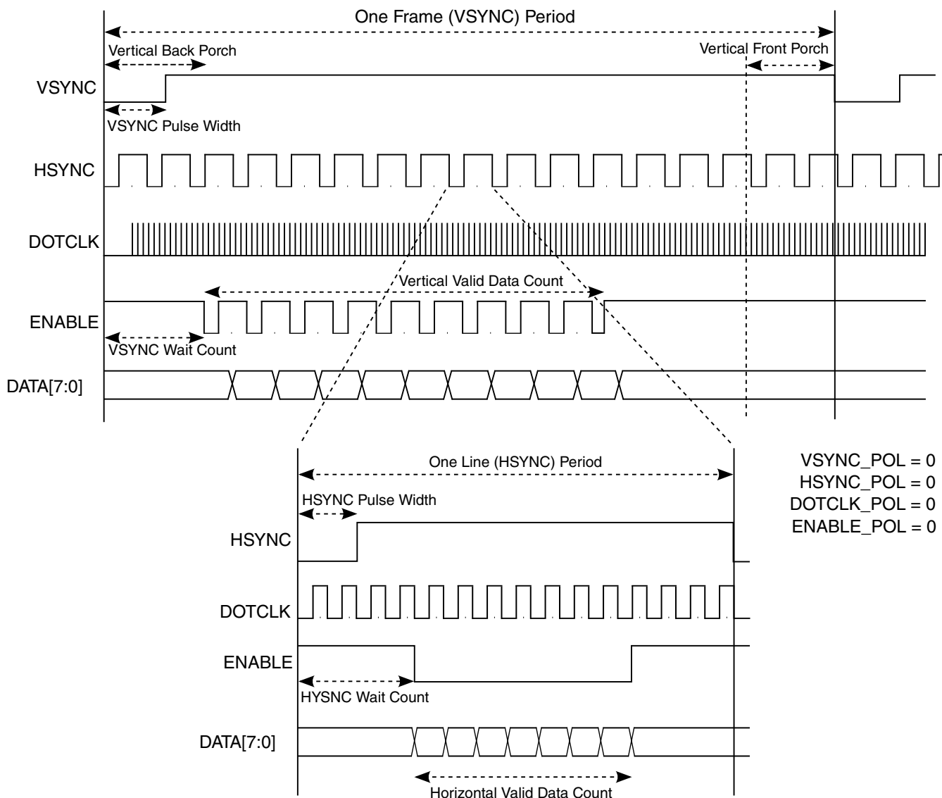
Figure 34-7. DOTCLK protocol with programmable parameters
