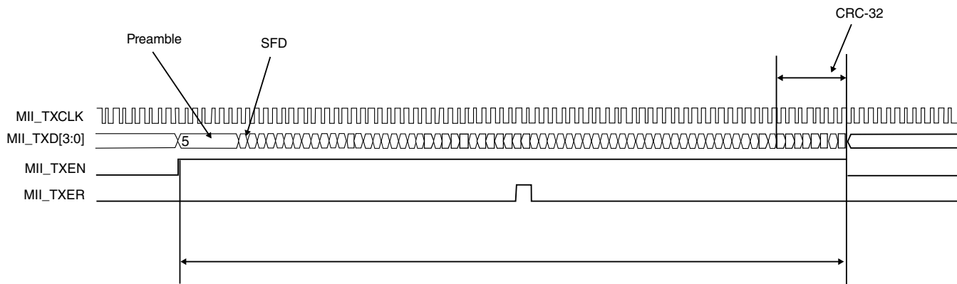
Figure 40-23. MII transmit operation — errored frame
