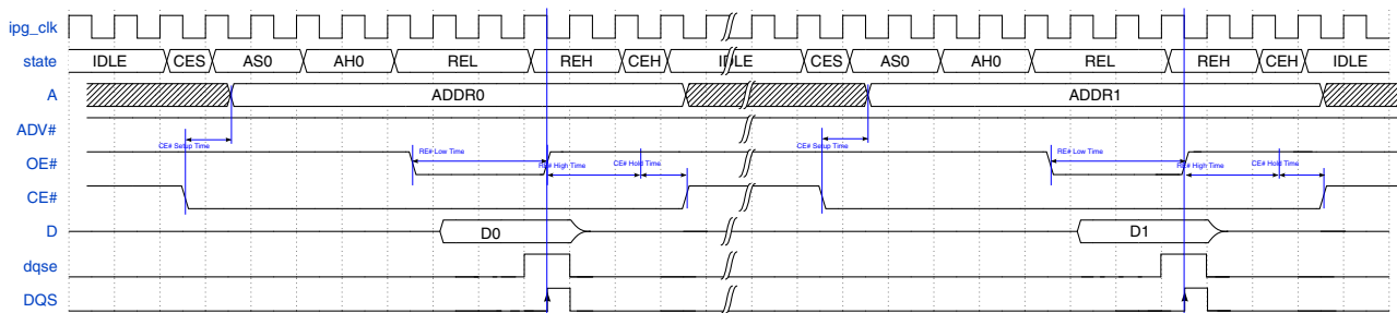
Figure 24-47. Flash Read in ASYNC mode (Non-ADMUX)
