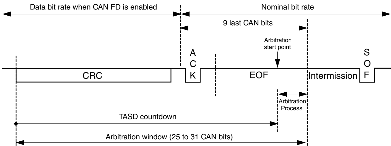
Figure 44-13. Optimal Tx Arbitration start point
