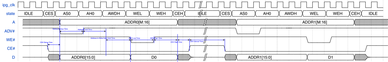
Figure 24-51. Flash Write in ASYNC mode (ADMUX)
