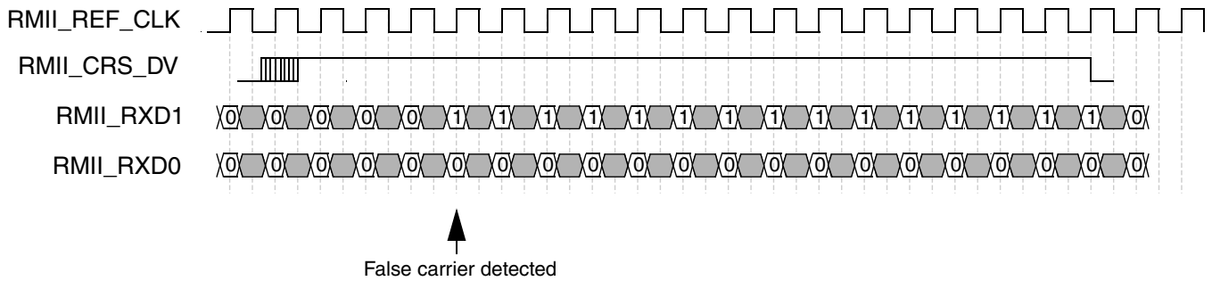
Figure 40-20. RMII receive operation with false carrier
