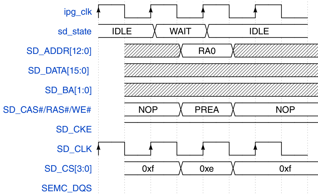
Figure 24-7. IP command - SDRAM PRECHARGE ALL
