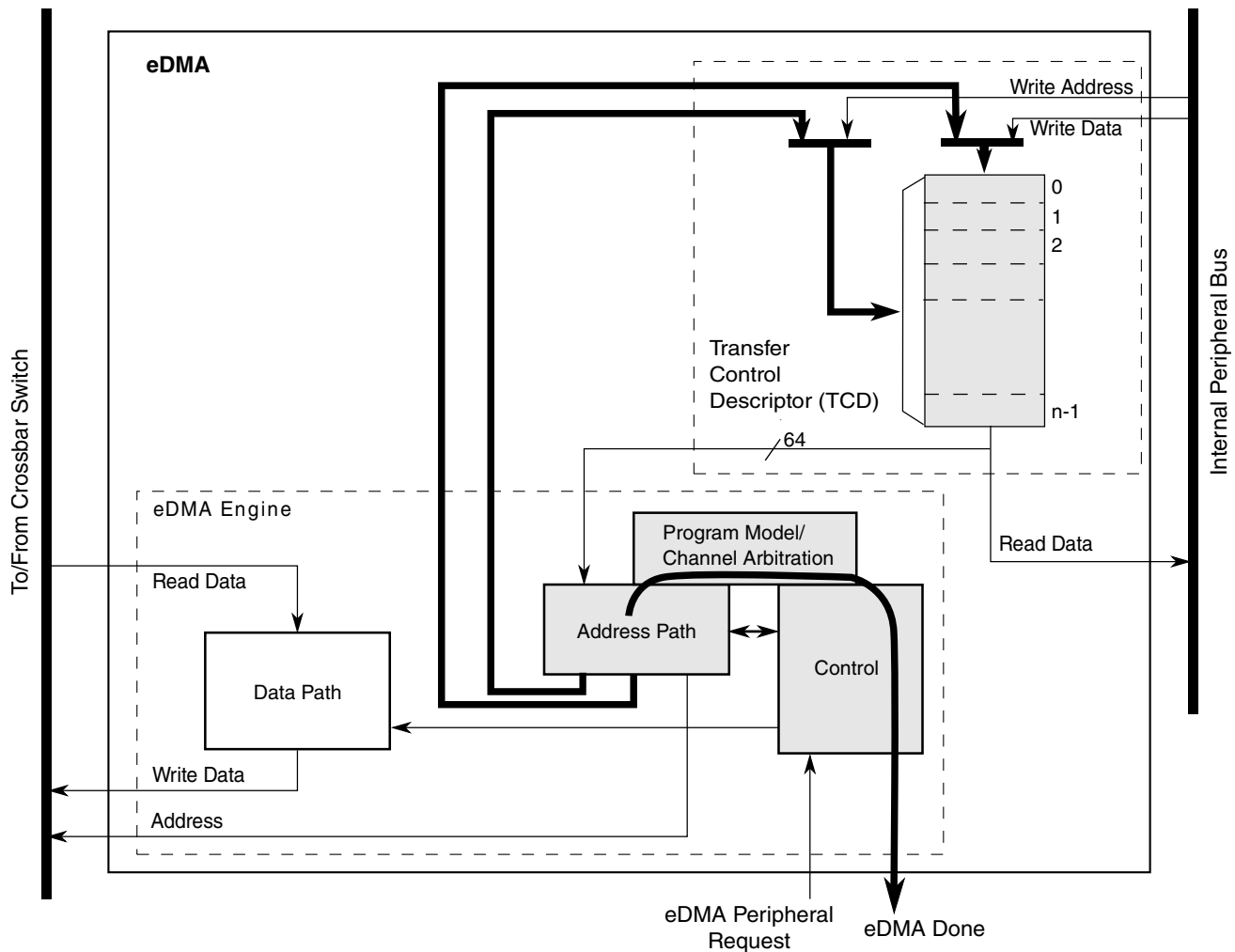
Figure 5-4. eDMA operation, part 3
