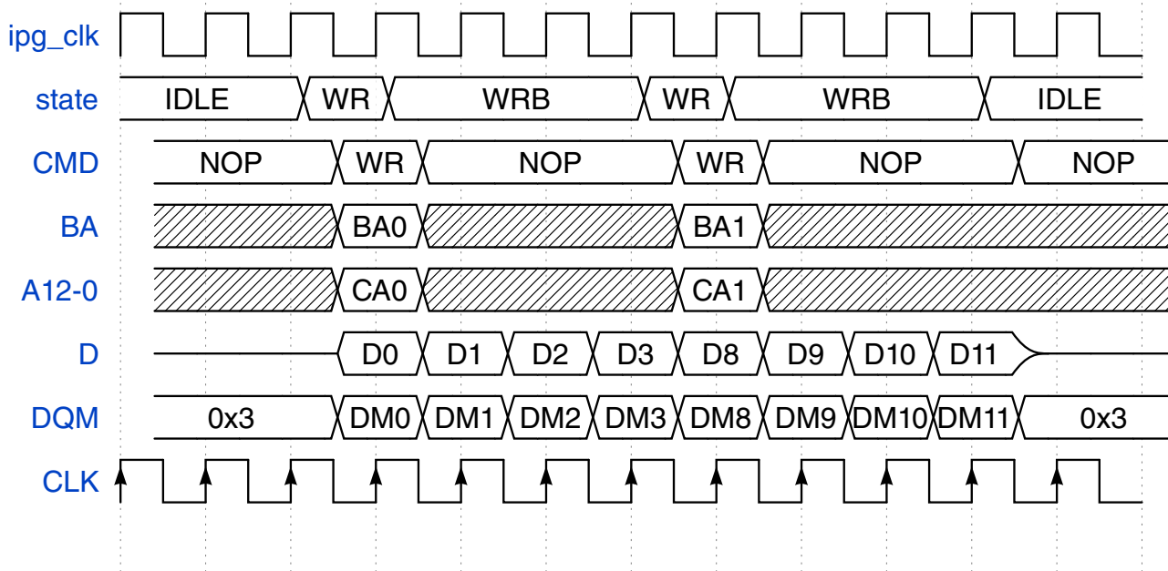
Figure 24-21. SDRAM Write-to-Write access
