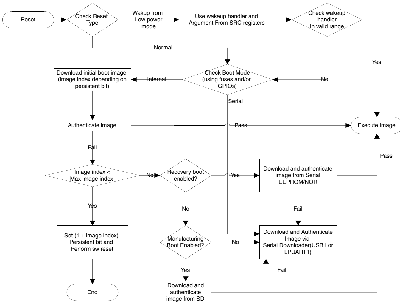
Figure 8-1. Boot flow
