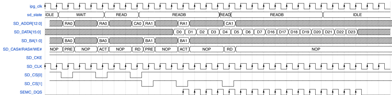
Figure 24-13. AXI command - Pipelined SDRAM Read
