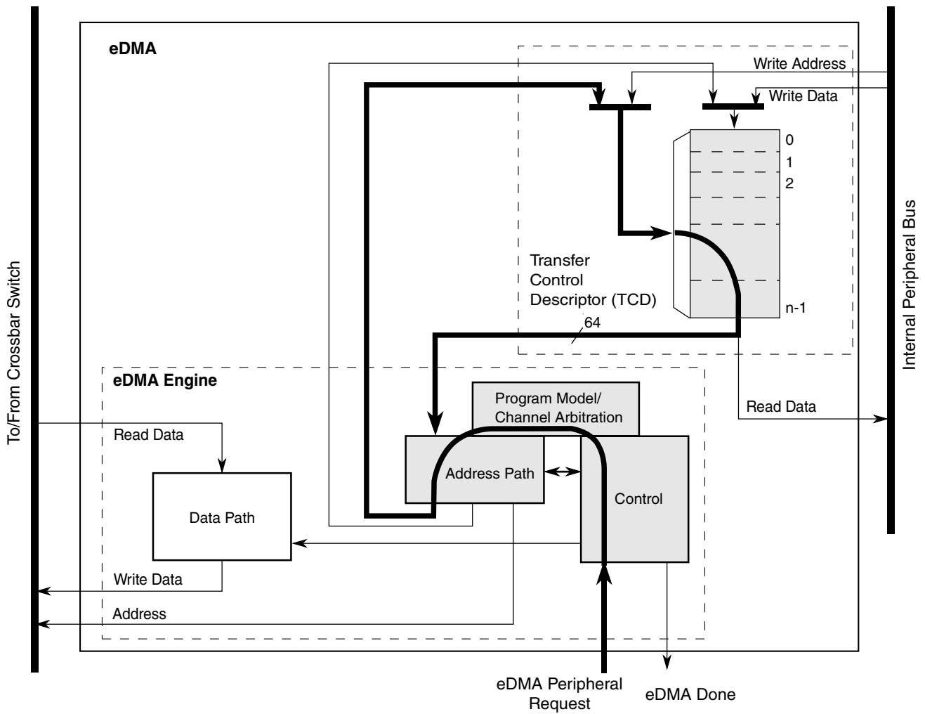
Figure 5-2. eDMA operation, part 1
