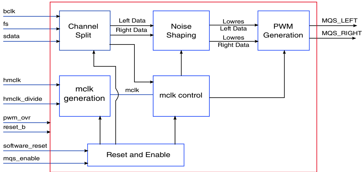
Figure 38-1. Block Diagram
