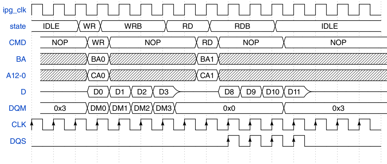
Figure 24-22. SDRAM Write-to-Read access (CL=1)
