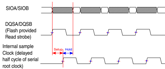
Figure 26-33. Input Timing 2 for Flash provided read strobe in SDR mode
