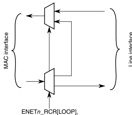
Figure 40-13. Loopback options
