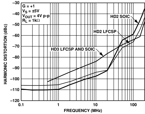
Figure 18. Harmonic Distortion vs. Frequency for Various Packages
