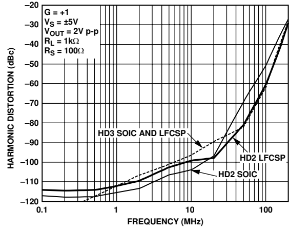
Figure 17. Harmonic Distortion vs. Frequency for Various Packages
