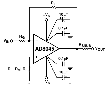
Figure 62. Inverting Configuration
