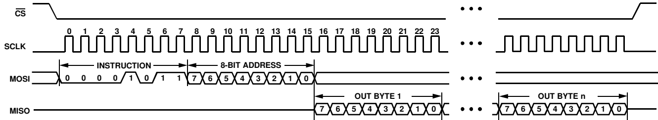
Figure 38. Burst Read
