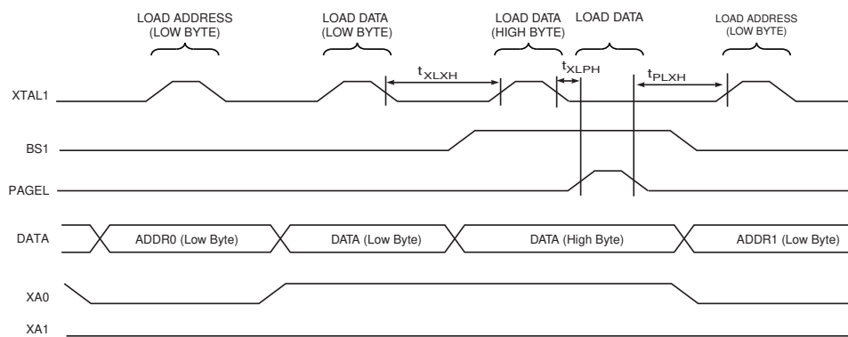
Figure 26-9. Parallel Programming Timing, Loading Sequence with Timing Requirements (1)
