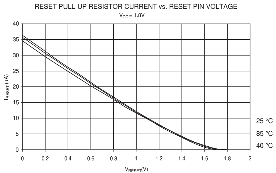
Figure 27-156. Reset Pull-up Resistor Current vs. Reset Pin Voltage ( V_{CC} = 1.8\text{ V} ).
