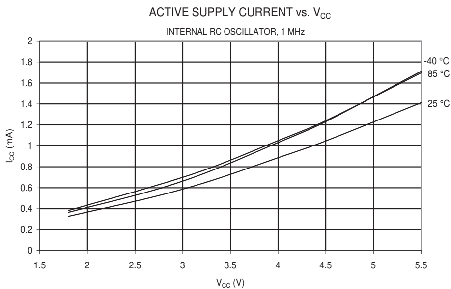
Figure 27-50. Active Supply Current vs. V_{CC} (Internal RC Oscillator, 1 MHz).
