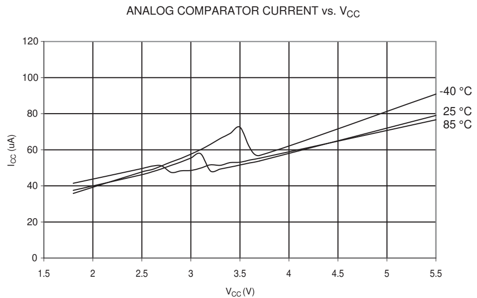
Figure 27-178. Analog Comparator Current vs. V_{CC} .
