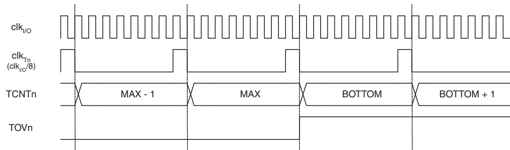
Figure 12-9. Timer/Counter Timing Diagram, with Prescaler ( f_{\text{clk}_{I/O}}/8 )
