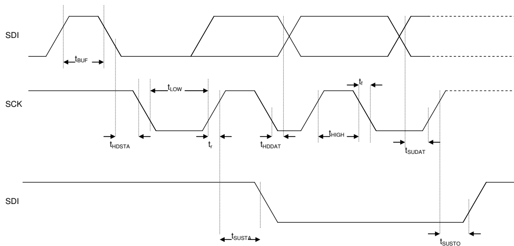
Figure 14: I²C timing diagram
