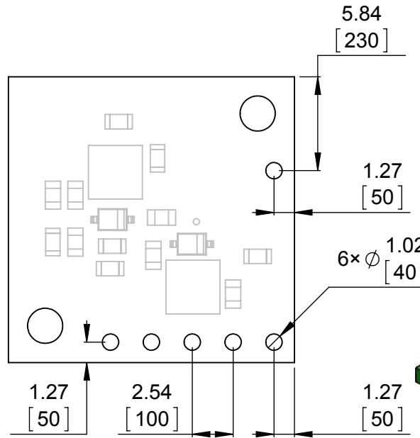
② Connector callouts (bottom view) Scale 3:1
