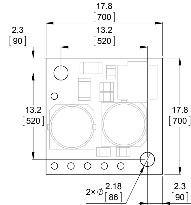
① Board dimensions (top view) Scale 3:1
