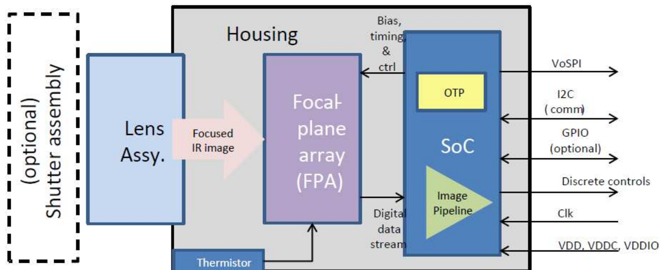
Figure 2 - Lepton Architecture
