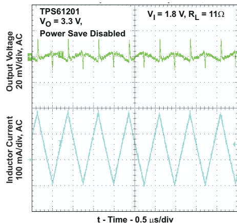
Figure 16. Output Voltage, Power Save Mode Disabled
