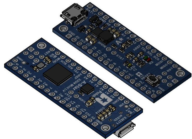
③ Isometric view Scale 3:2
