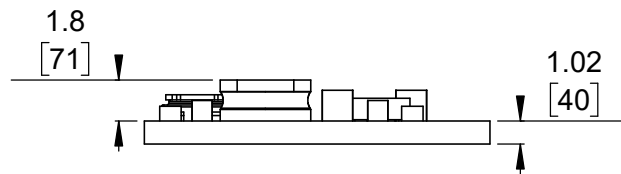
⑤ Profile Scale 3:1
