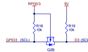
Dedicated I2C bidirectional shifters
